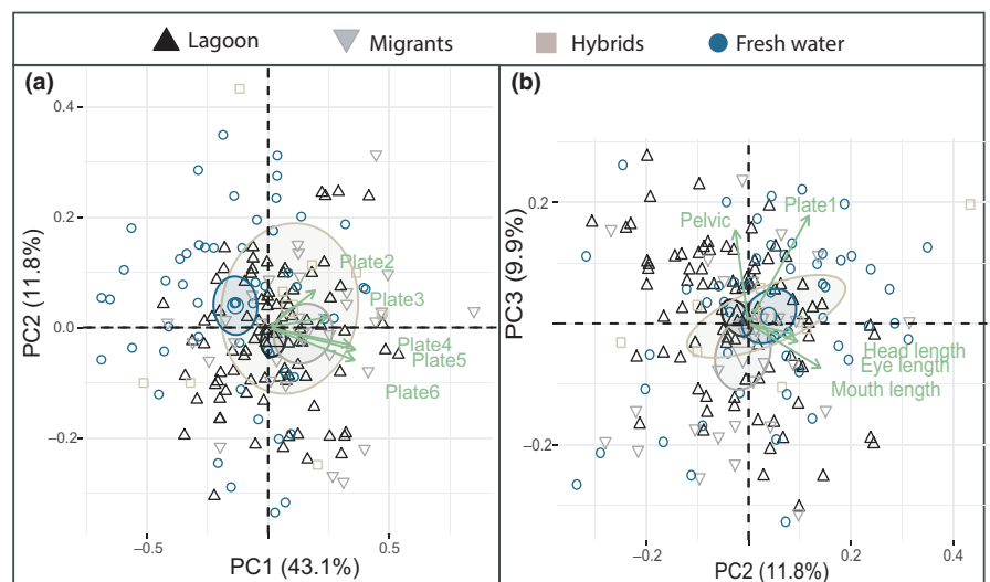
FIGURE 7 PCA for the lagoon, the migrants, the hybrids, and the freshwater population. a) illustrates PC1 plotted against PC2 for all traits, and b) illustrates PC2 plotted against PC3 for all traits. Both plots include the five most influential variables in green. The lagoon fish are plotted in black triangles, the migrants in gray triangles, the hybrids in light brown squares, and the fresh water in blue circles
