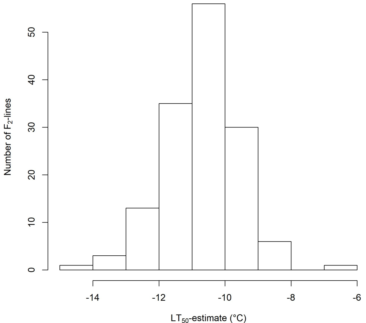
Fig 2. Progeny of 'NCGR1363' × 'Alta' show a "normal" distribution of freeze tolerance. Histogram of the LT_{50} estimated values calculated for the progeny of the selfed 'NCGR1363' × 'Alta' mapping population ( n = 142 ). LT_{50} estimates are given in °C.
